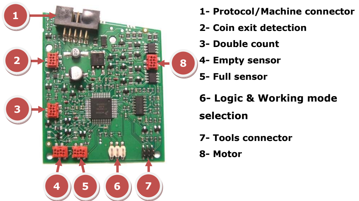
Figure 1. Parallel control board
