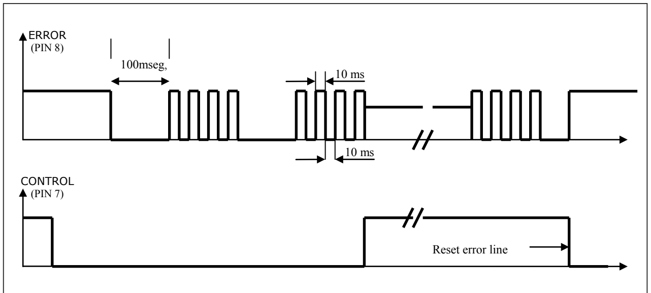
Figure 7. Negative logic
