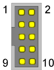
Fig. 10 Position of the connecting pins (EMP plug)
