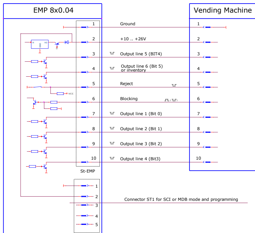
Fig. 30 Connecting diagram EMP 8x0.04 v7
