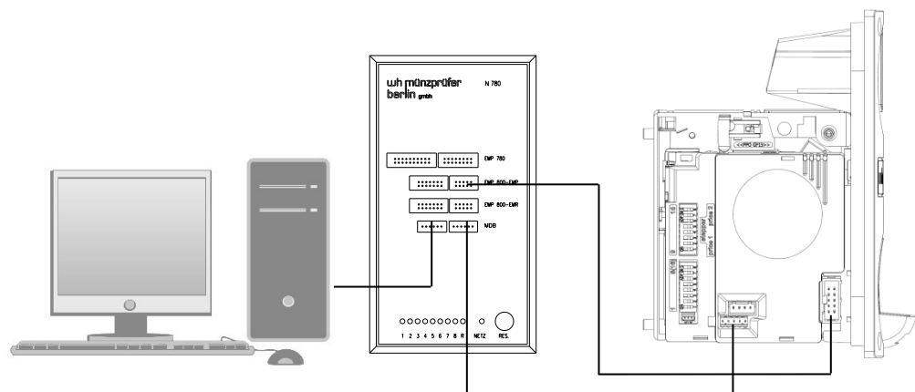
Fig. 3 Connection of the coin selector with the N 780 and the PC
