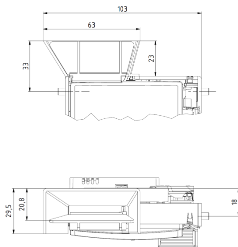
Fig. 15 Coin funnel (Option /F)
