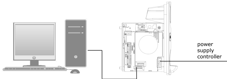
Fig. 4 Connection between a coin operated machine controller, an installed coin selector and a PC
