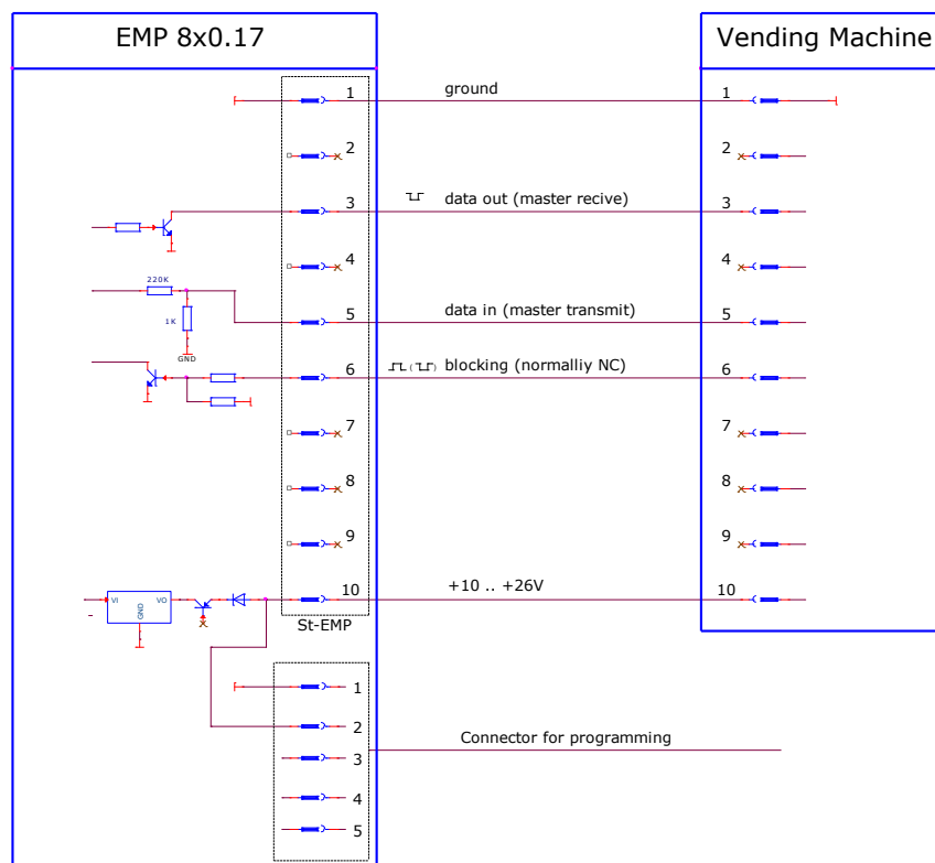
Fig. 32 Connecting diagram EMP 8x0.17 v7 with 10-pole MDB Interface
