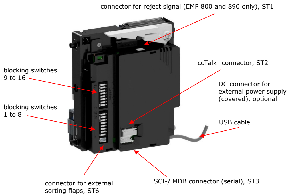
Fig. 27 Location of connectors and control elements EMP 8x0.14 v7
