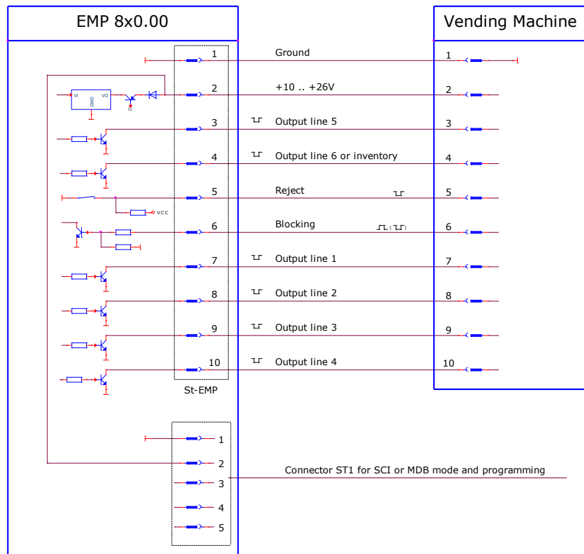
Fig. 29 Connecting diagram EMP 8x0.00 v7
