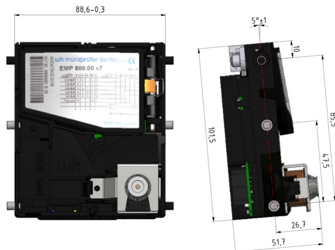
Fig. 1 EMP 8x0 v7 – Dimensions and Positioning
