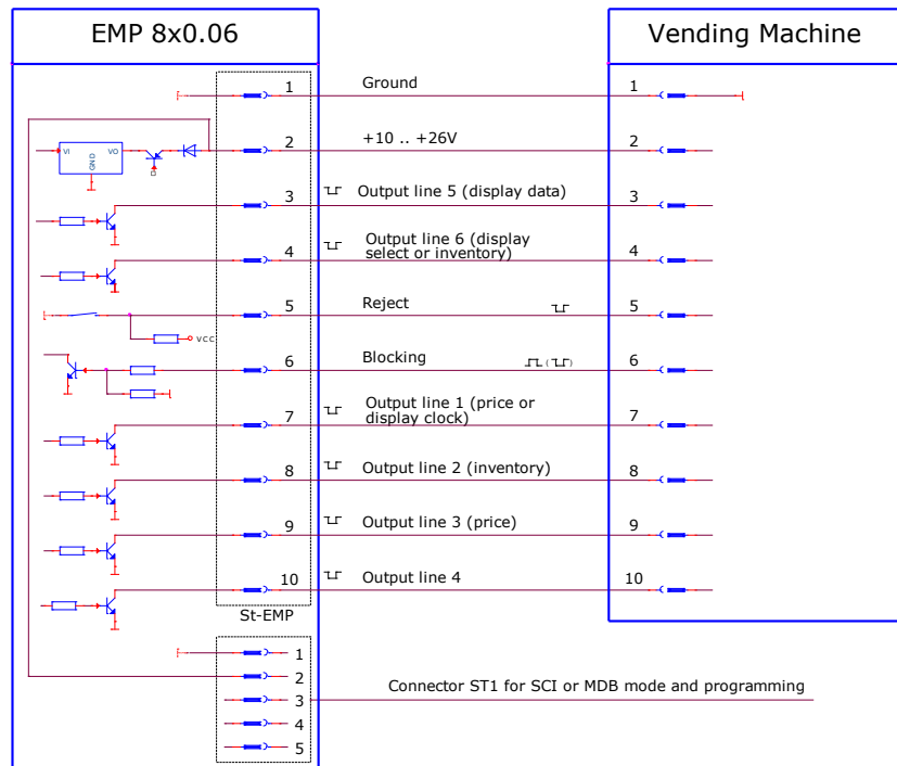
Fig. 31 Connecting diagram EMP 8x0.06 v7
