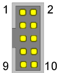
Fig. 17 Position of the connecting pins (EMP plug)
